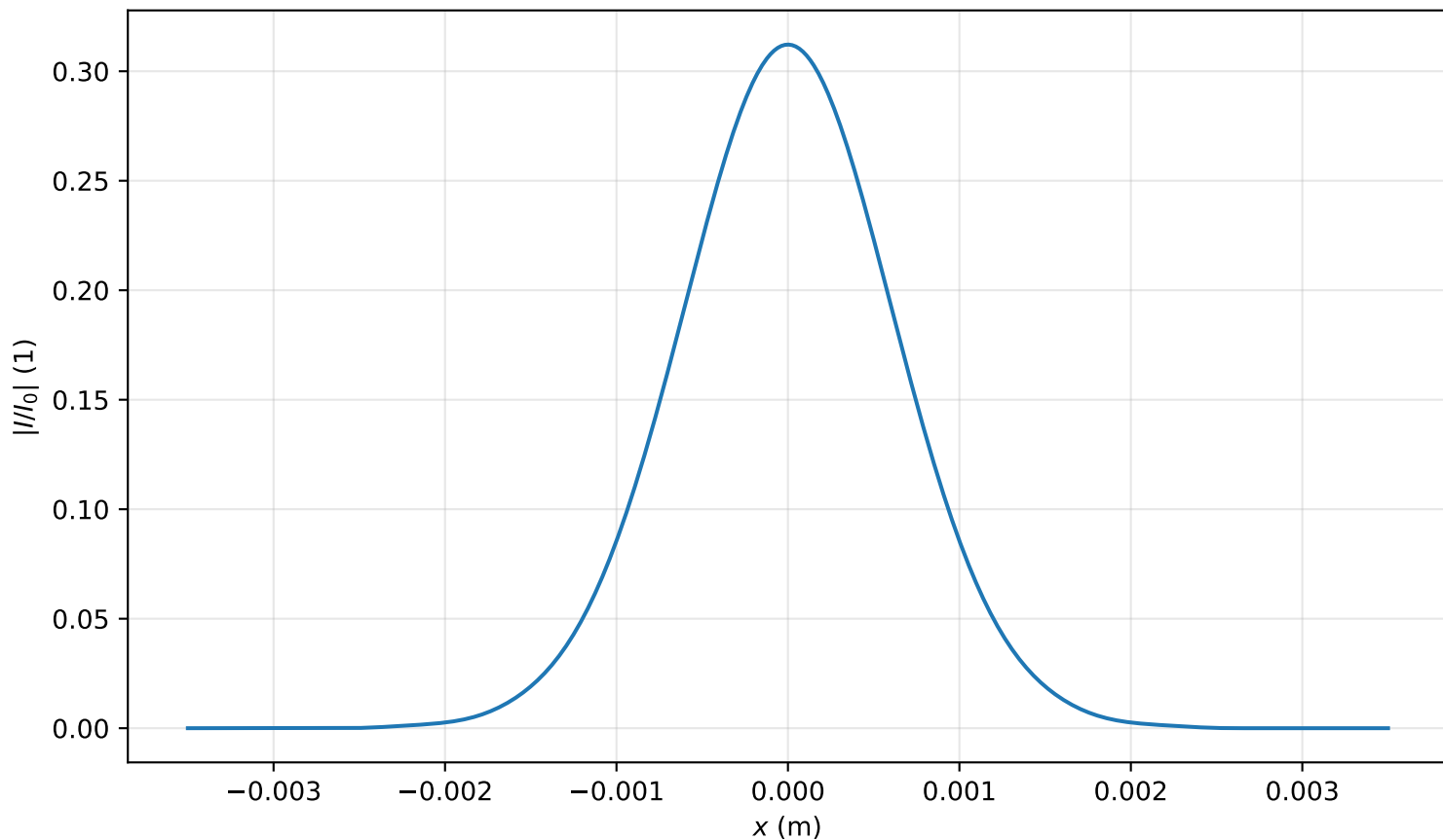
Intensity profile I(x, y = 0, z = 3.423m)/I_0 , P_{in}=0.2P_{cr} , artificial time
